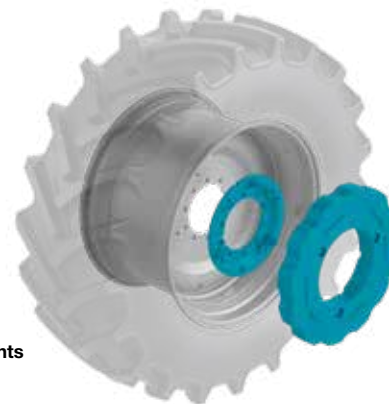
Counterweight 600kg
